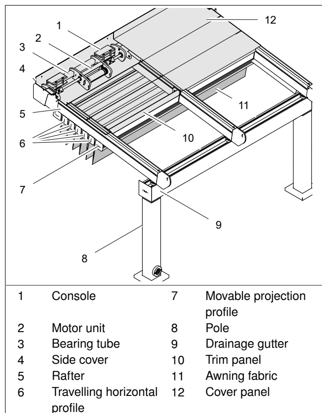
Fig. 1: Parts overview of pergola awning Perea P70
